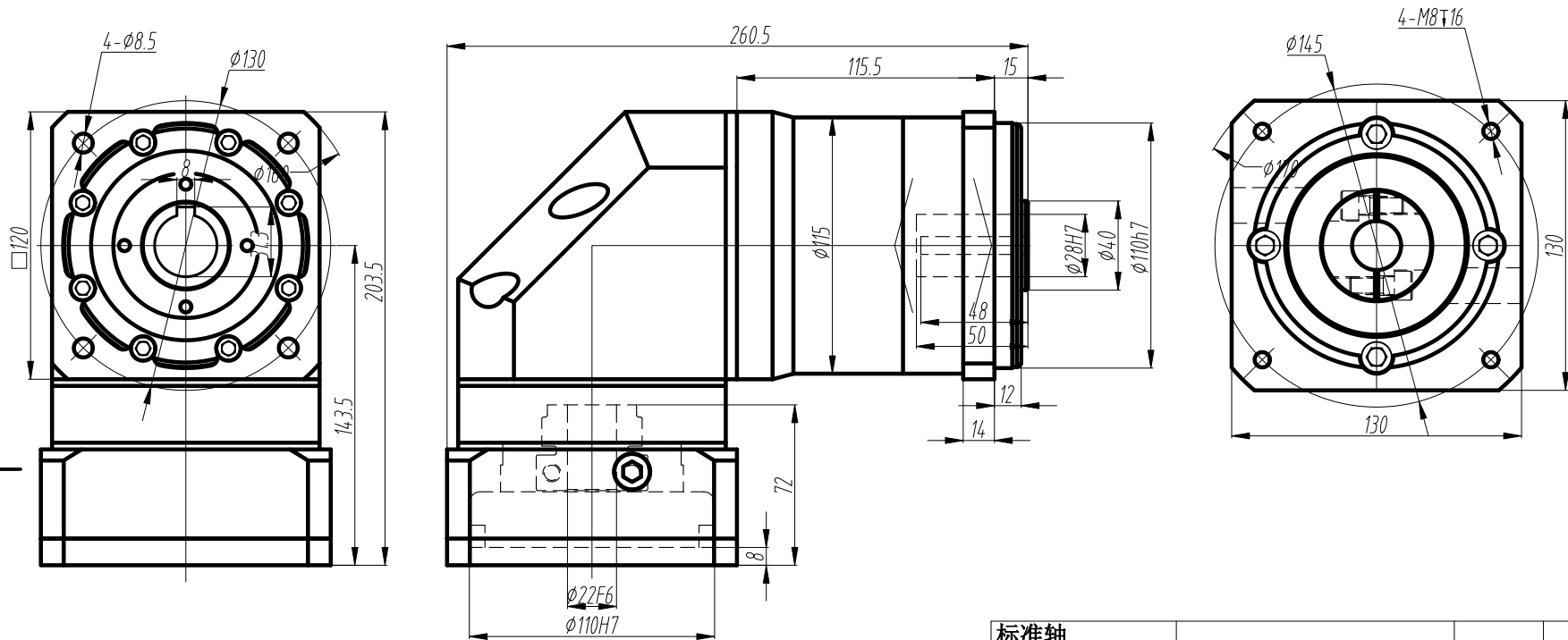
标准轴 Standard output shaft
